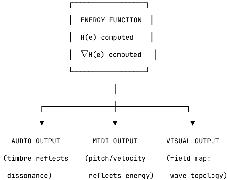
Figure 4. The Soma-Field Instrument: input, computation, and multimodal output.
