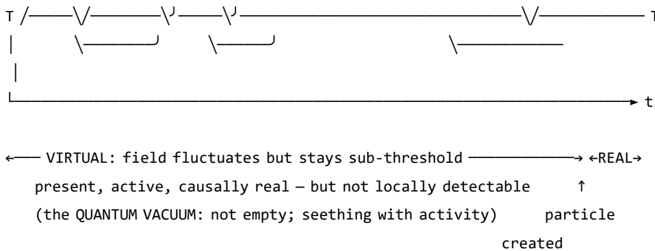
Figure 0. A single field mode in quantum field theory. The field oscillates continuously. Below the detection threshold T , excitations are sub-threshold — real and causally active, but not detectable as particles. The quantum vacuum is not empty; it is a field in constant motion that never quite crosses the threshold. When the amplitude does cross T , a particle exists: a locally observable excitation. The same structure — field always present, consciousness only when threshold crossed — is the core of the Soma-Field Model.
