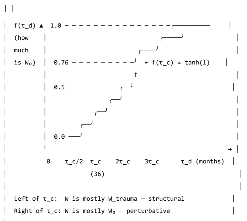
Figure 6.1. The structural fraction f(\tau_d) . This function describes what proportion
