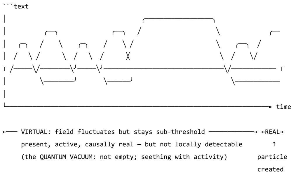
Figure 0. A single field mode in quantum field theory. The field oscillates continuously. Below the detection threshold T , excitations are sub-threshold — real and causally active, but not detectable as particles. The quantum vacuum is not empty; it is a field in constant motion that never quite crosses the threshold. When the amplitude does cross T , a particle exists: a locally observable excitation. The same structure — field always present, consciousness only when threshold crossed — is the core of the Soma-Field Model.
