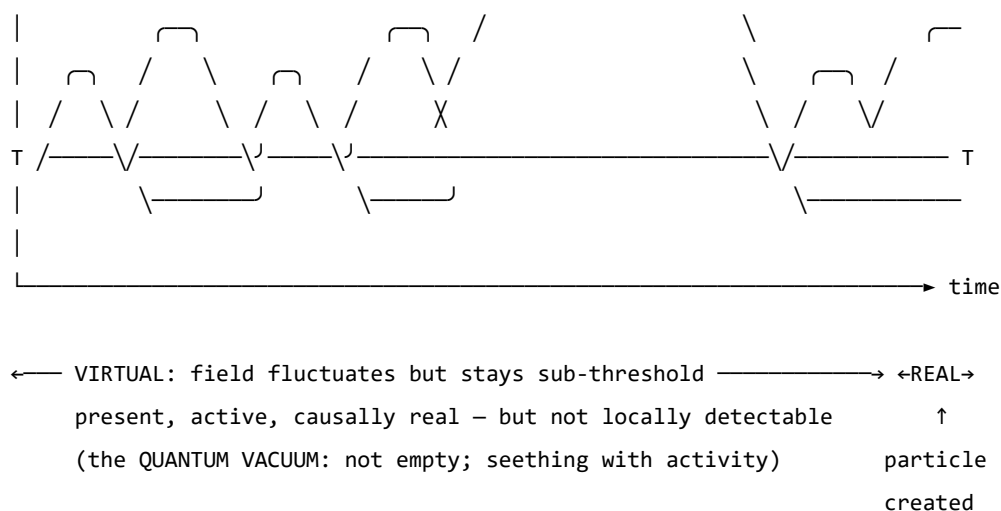
Figure 0. A single field mode in quantum field theory. The field oscillates continuously. Below the detection threshold T , excitations are sub-threshold — real and causally active, but not detectable as particles. The quantum vacuum is not empty; it is a field in constant motion that never quite crosses the threshold. When the amplitude does cross T , a particle exists: a locally observable excitation. The same structure — field always present, consciousness only when threshold crossed — is the core of the Soma-Field Model.
