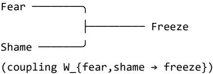
EMOTIONAL INTERACTION AS FEYNMAN VERTEX
