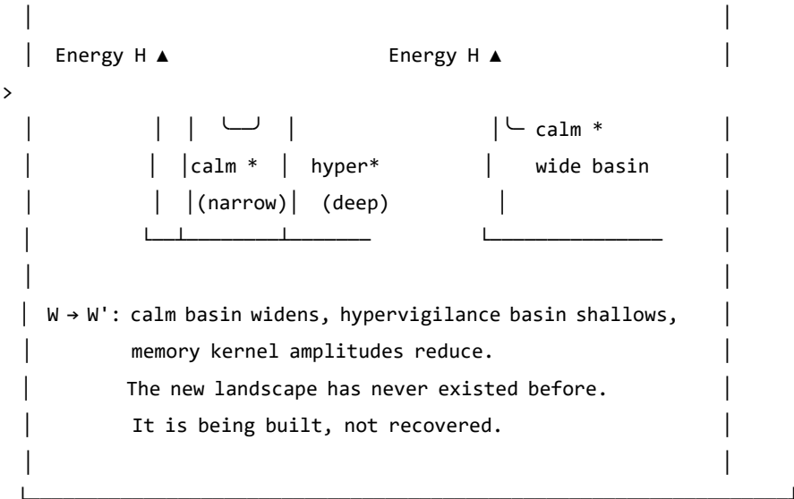
Figure 10.1. Forward transformation. The target W' is not a reconstruction of a prior baseline (which may not have existed). It is a new configuration with desired dynamical properties: a wide calm basin, shallow hypervigilance attractor, and reduced memory kernel amplitudes. The path from W to W' uses therapeutic tools as the mechanism of landscape modification.
