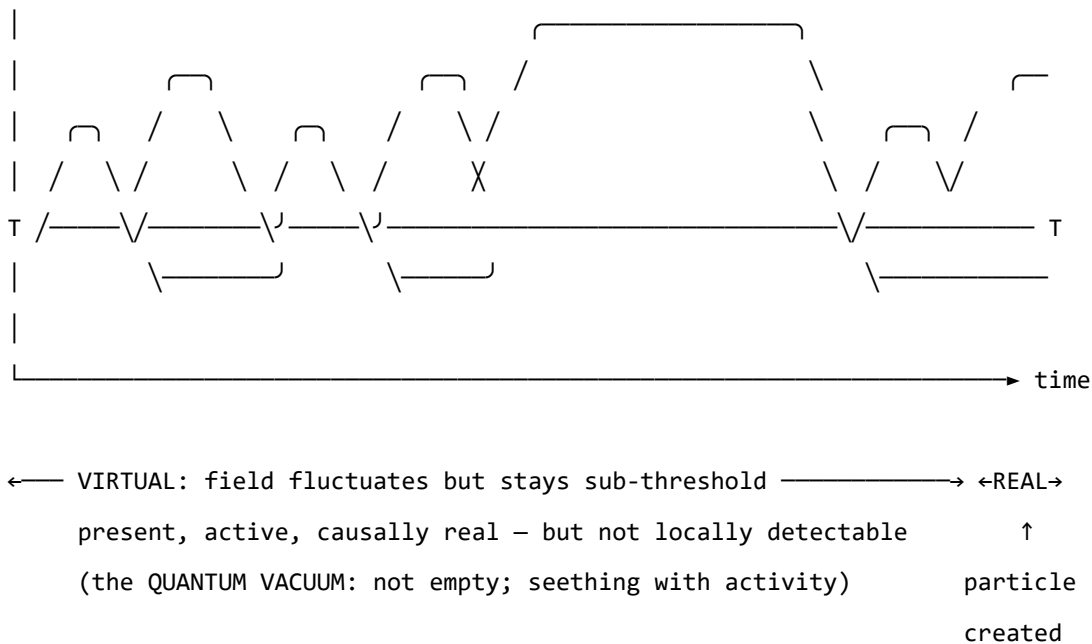
Figure 0. A single field mode in quantum field theory. The field oscillates continuously. Below the detection threshold T , excitations are sub-threshold — real and causally active, but not detectable as particles. The quantum vacuum is not empty; it is a field in constant motion that never quite crosses the threshold. When the amplitude does cross T , a particle exists: a locally observable excitation. The same structure — field always present, consciousness only when threshold crossed — is the core of the Soma-Field Model.
