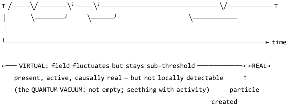
Figure o. A single field mode in quantum field theory. The field oscillates continuously. Below the detection threshold T , excitations are sub-threshold — real and causally active, but not detectable as particles. The quantum vacuum is not empty; it is a field in constant motion that never quite crosses the threshold. When the amplitude does cross T , a particle exists: a locally observable excitation. The same structure — field always present, consciousness only when threshold crossed — is the core of the Soma-Field Model.
