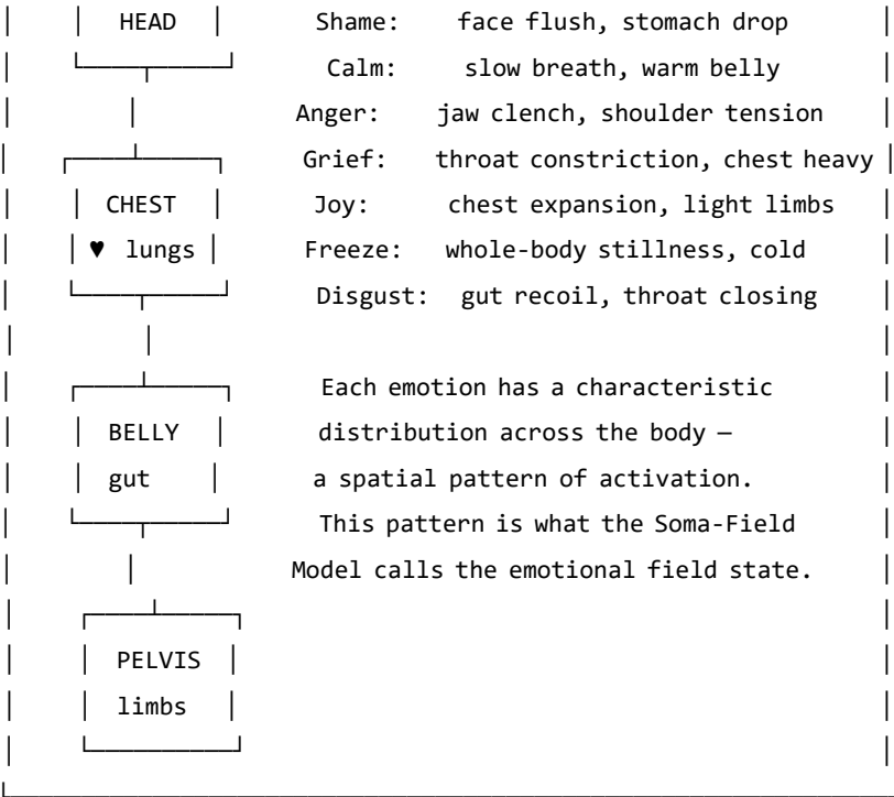
Figure 2.1. The body map of emotional activation. Emotions are not events in time, they are distributed patterns of physiological arousal across the body. Researcher Nummenmaa et al. (2014) mapped these patterns by asking participants to colour in silhouettes where they felt each emotion. The patterns are consistent across cultures.
