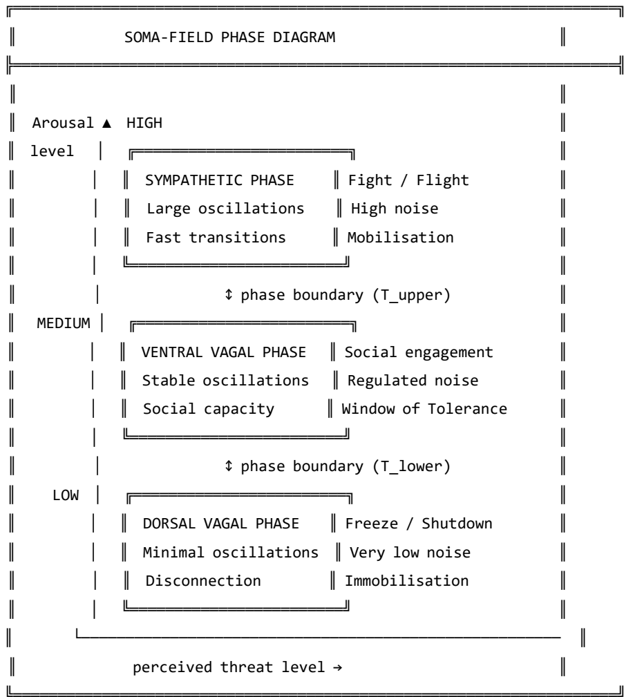
Figure 8.1. The nervous system as a phase diagram. Three distinct phases correspond to the three polyvagal states. Phase boundaries (T_upper and T_lower) mark the transitions. For a regulated nervous system, most experience occurs in the ventral
