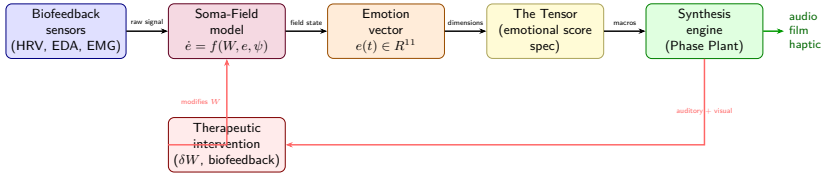
Figure 8: Figure 9.2. The Soma-Field instrument pipeline. Biofeedback sensors (HRV, EDA, EMG) feed the soma-field model, which produces a real-time emotion vector \mathbf{e}(t) \in \mathbb{R}^{1,1} . This drives The Tensor (the emotional score specification), which controls a synthesis engine (Phase Plant). A feedback loop via therapeutic intervention \delta W allows the practitioner to modify the coupling matrix directly — closing the loop between measurement and treatment. Author's original figure.
