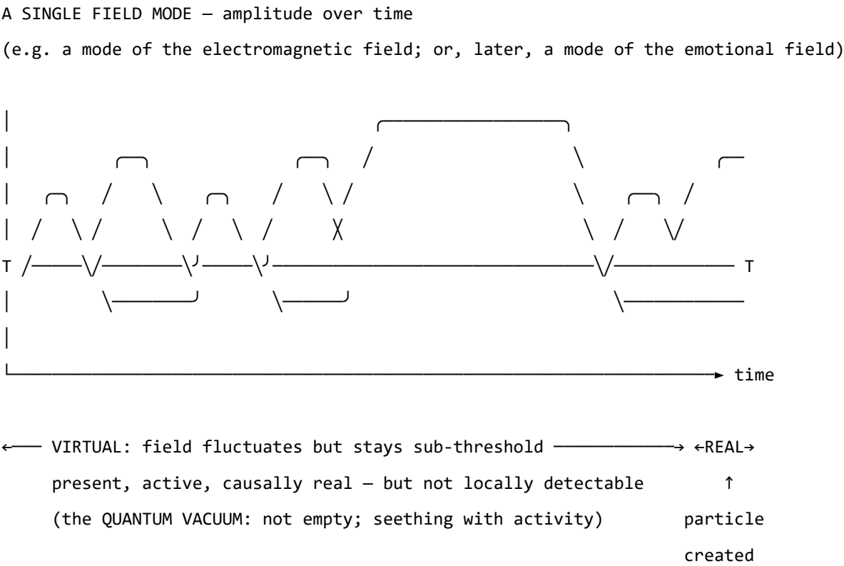
Figure 0. A single field mode in quantum field theory. The field oscillates continuously. Below the detection threshold T , excitations are sub-threshold — real and causally active, but not detectable as particles. The quantum vacuum is not empty; it is a field in constant motion that never quite crosses the threshold. When the amplitude does cross T , a particle exists: a locally observable excitation. The same structure — field always present, consciousness only when threshold crossed — is the core of the Soma-Field Model.
