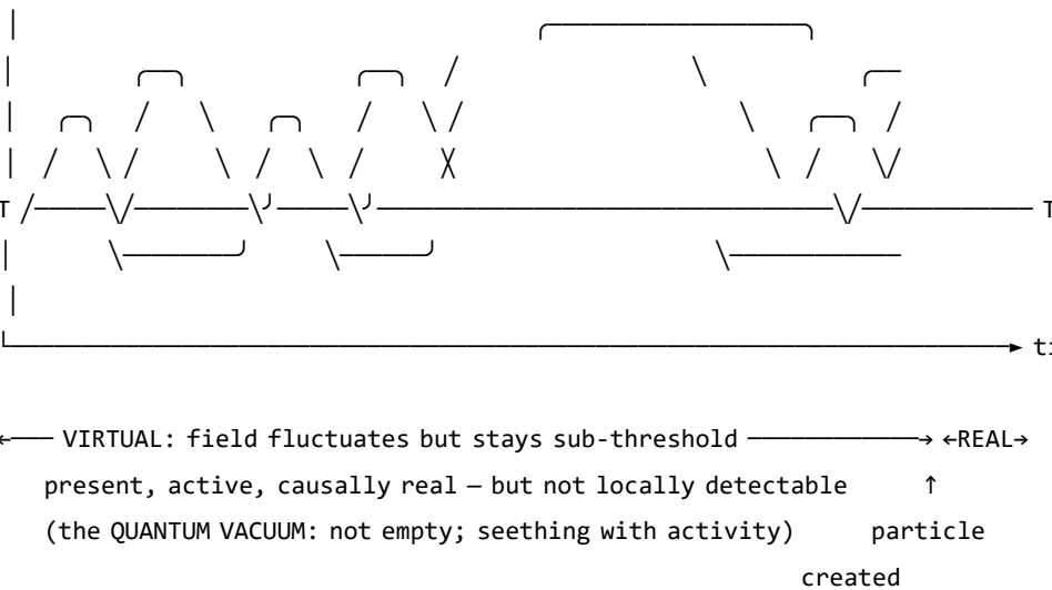
Figure 0. A single field mode in quantum field theory. The field oscillates continuously. Below the detection threshold T , excitations are
