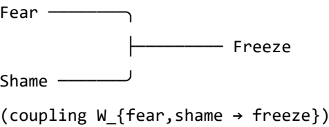
EMOTIONAL INTERACTION AS FEYNMAN VERTEX
