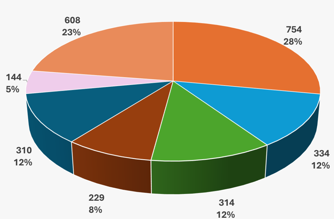
Minor Minerals
