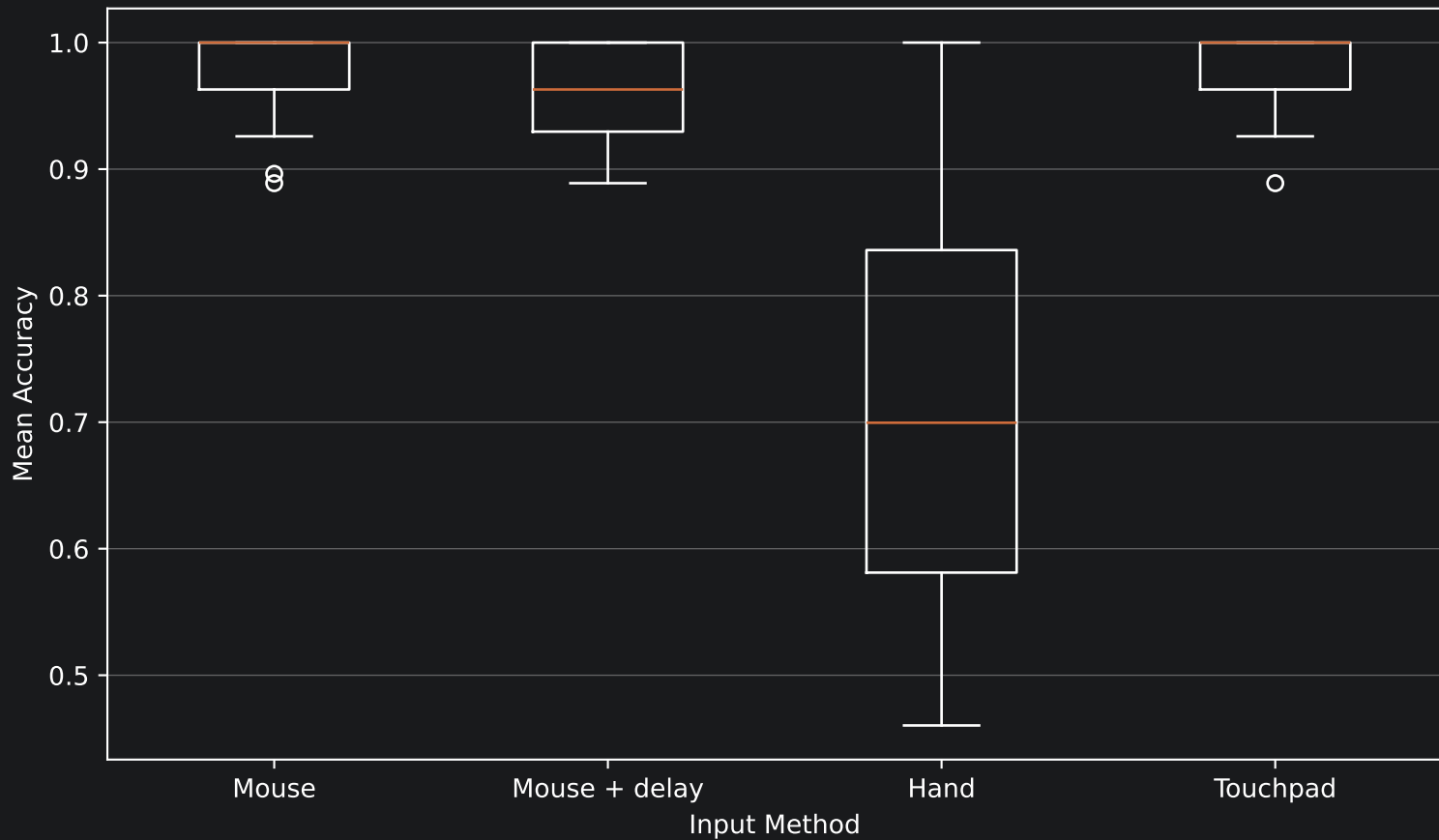
Accuracy by Input Method
