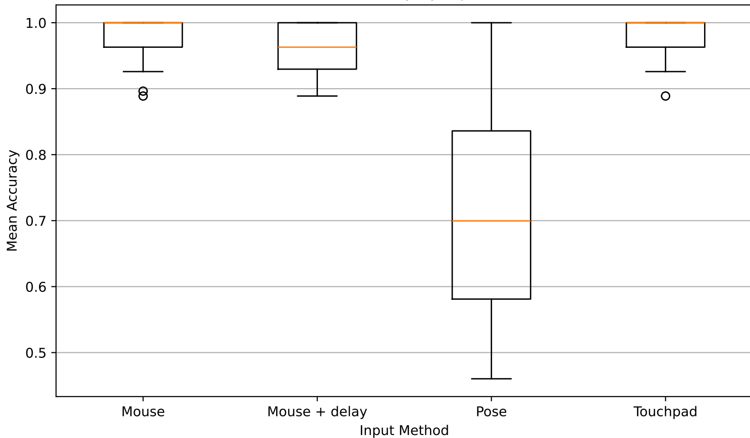
Fitts Task: Accuracy by Input Method
