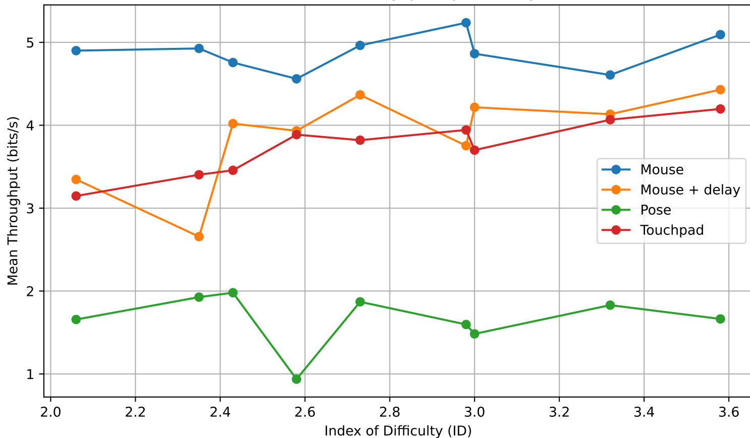
Fitts Task: Throughput by Difficulty
