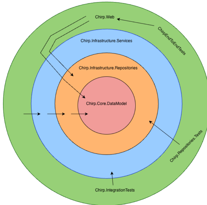
Figure 2: Onion Architecture
