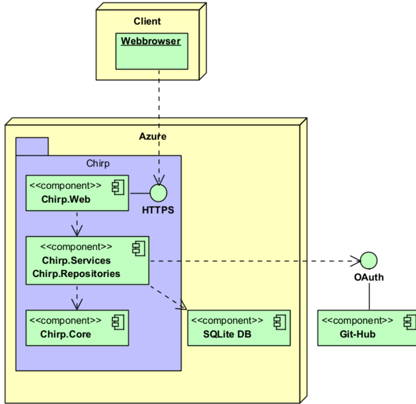
Figure 3: Deployed Components
