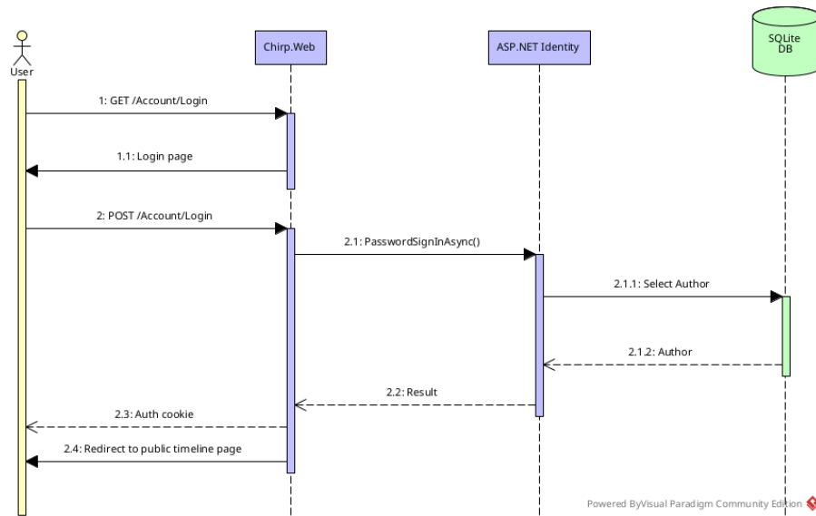
Figure 8: Login sequence
