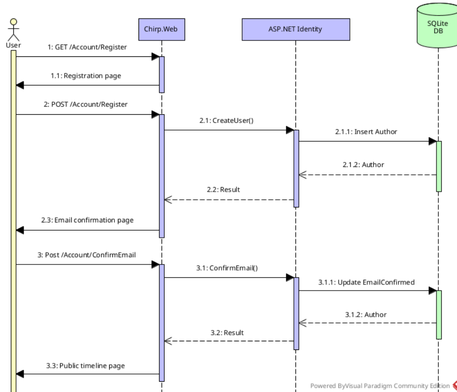
Figure 6: Register sequence
