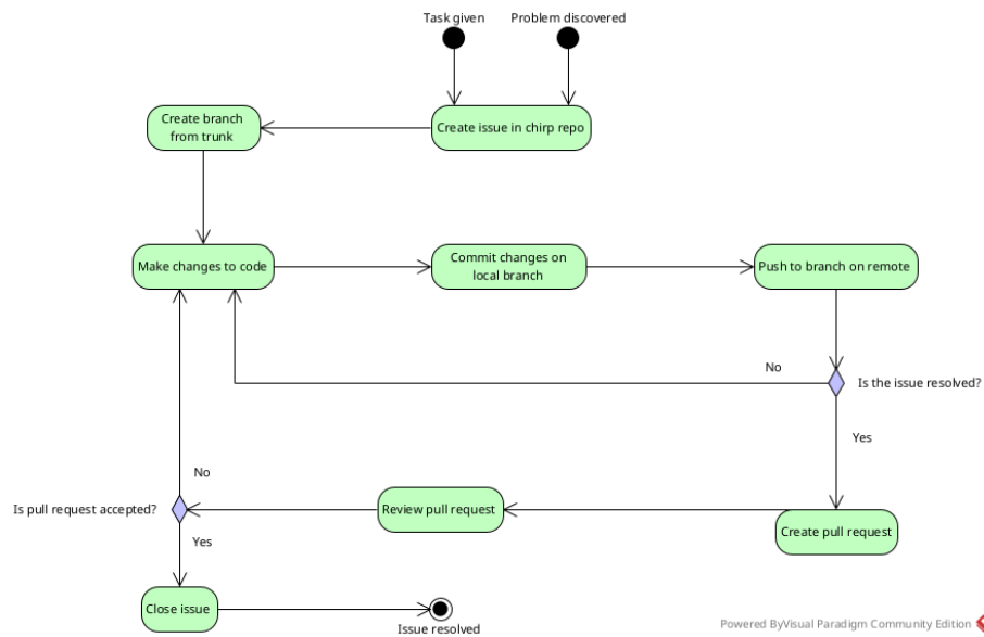
Figure 17: Flow diagram from issue creation to resolution
