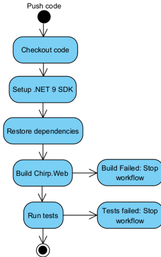
Figure 13: Build and Test workflow
