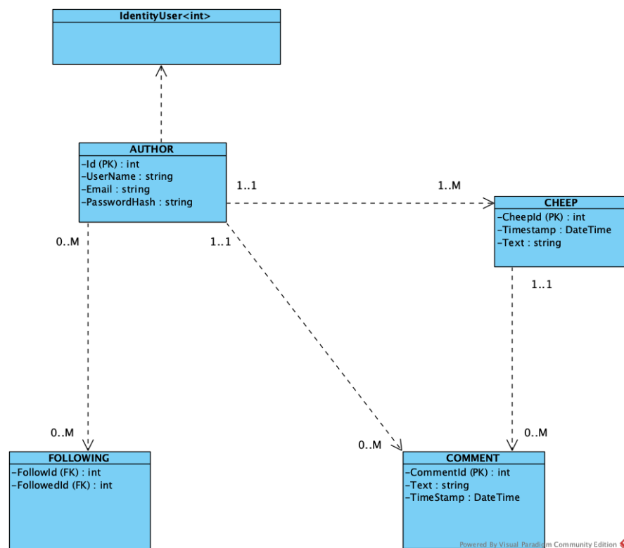
Diagram 1.1: Domain Model.
