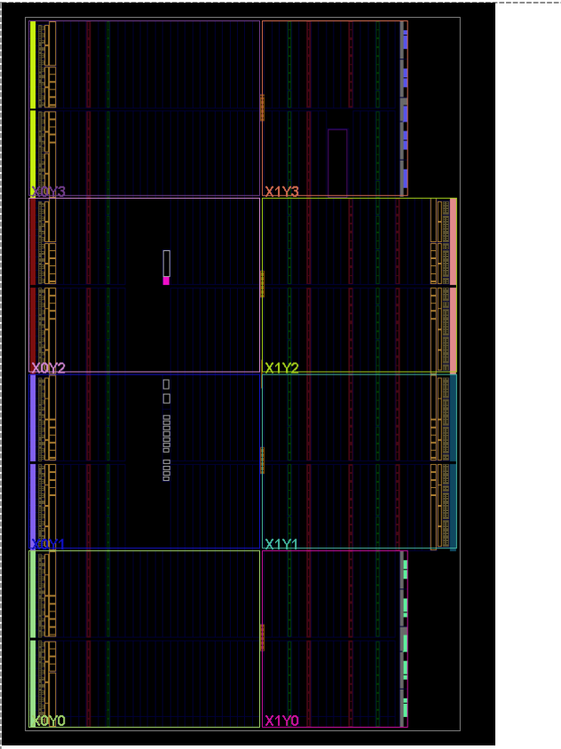
Fig. 4. Post-implementation device view (clock regions X0Y0 to X1Y3, Nexys4 DDR / xc7a100t).
