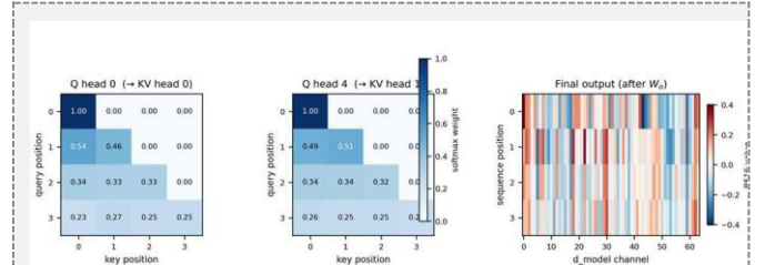
Fig. 5. Golden-model reference output for a representative test case ( seq\_len=4 , d\_model=64 , 8 Q / 2 KV heads, causal mask): softmax attention weights for two Q heads, and the final projected output, from the Python/BF16 golden model. Individual RTL stages now match this model's per-operation behavior at the module level (Section X). A matching full end-to-end ( top.sv ) RTL run against this exact reference is still pending.
