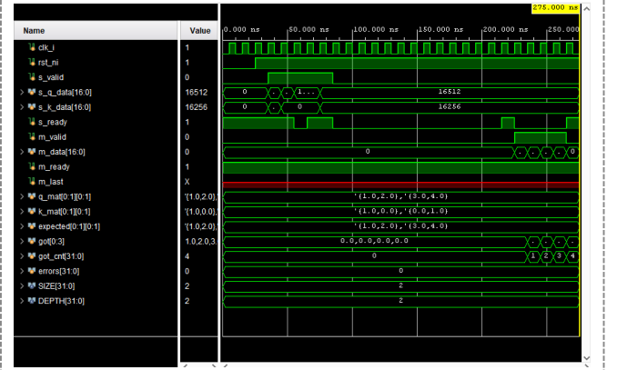
Fig. 3. Waveform from tb_qk_array.sv, exercising the shared Q \cdot K^T / score- V systolic array through mod_a_wrapper against a hand-computed 2 \times 2 case ( Q = \begin{bmatrix} 1 & 2 \\ 3 & 4 \end{bmatrix} , identity K , so the expected result equals Q ). All four output elements match, errors = 0. m_last reads X (shown in red) because this unit test does not connect that port. It is simply unexercised here, not a fault.
