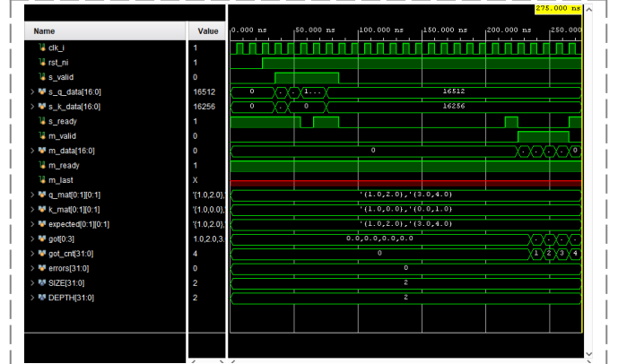
Fig. 3. Waveform from tb_qk_array.sv, exercising the shared Q \cdot K^T / \text{score} \cdot V systolic array through mod_a_wrapper against a hand-computed 2 \times 2 case ( Q = \begin{bmatrix} 1, 2 \\ 3, 4 \end{bmatrix} , identity K , so the expected result equals Q ). All four output elements match, errors = 0. m_last reads X (shown in red) because this unit test does not connect that port. It is simply unexercised here, not a fault.
