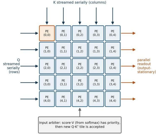
Figure 3. Output-stationary operation of the shared Q \cdot K^T / score-V systolic array.
