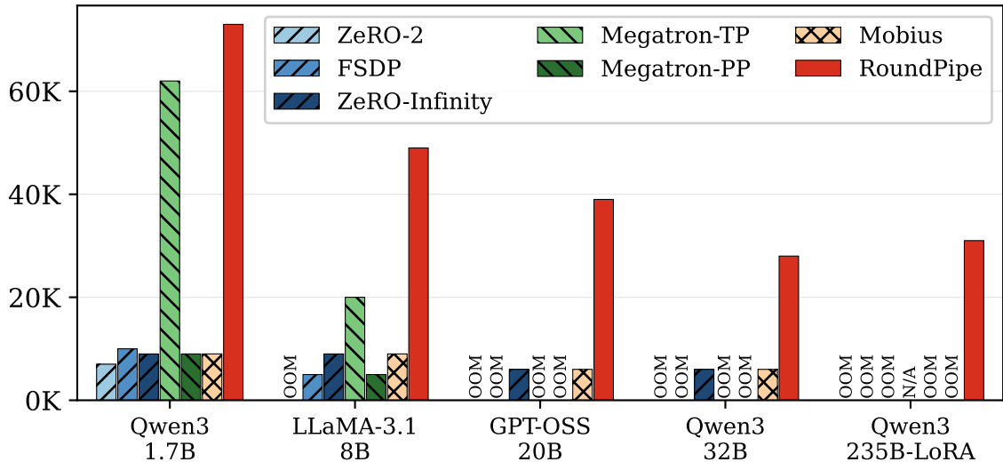
Max Sequence Length on 8×RTX 4090
