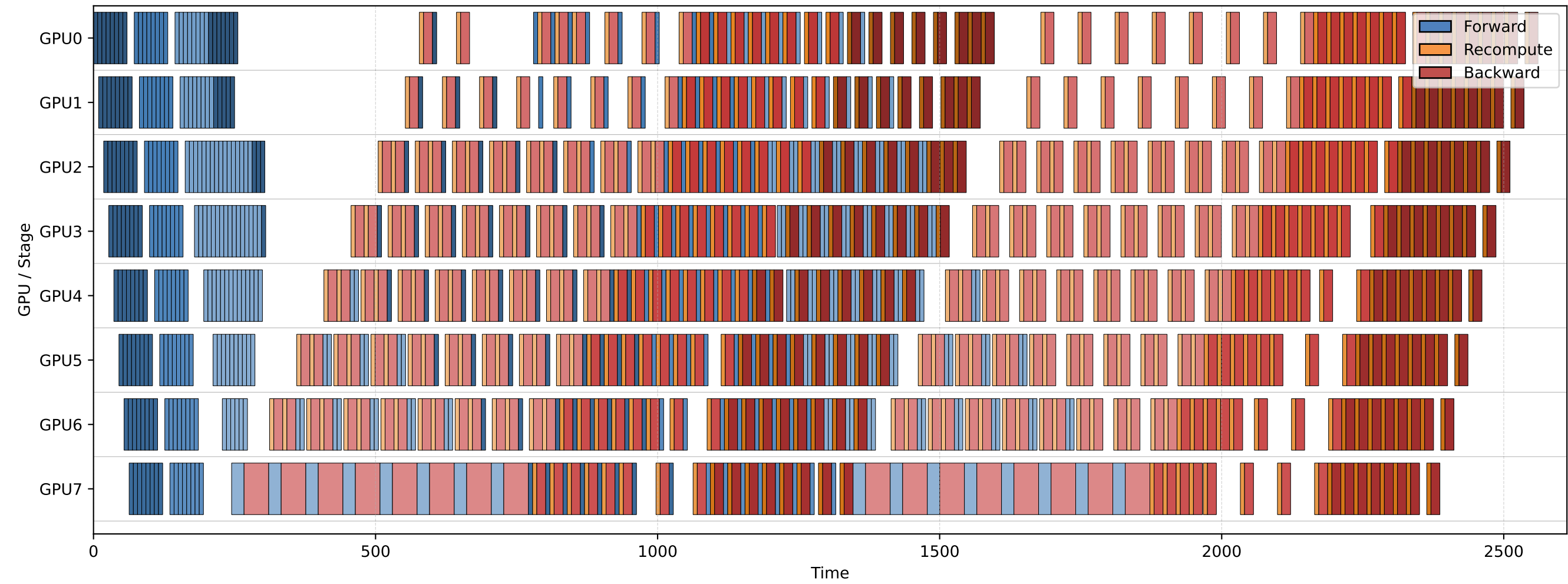
Qwen3-1.7B Interleaved-1F1B
