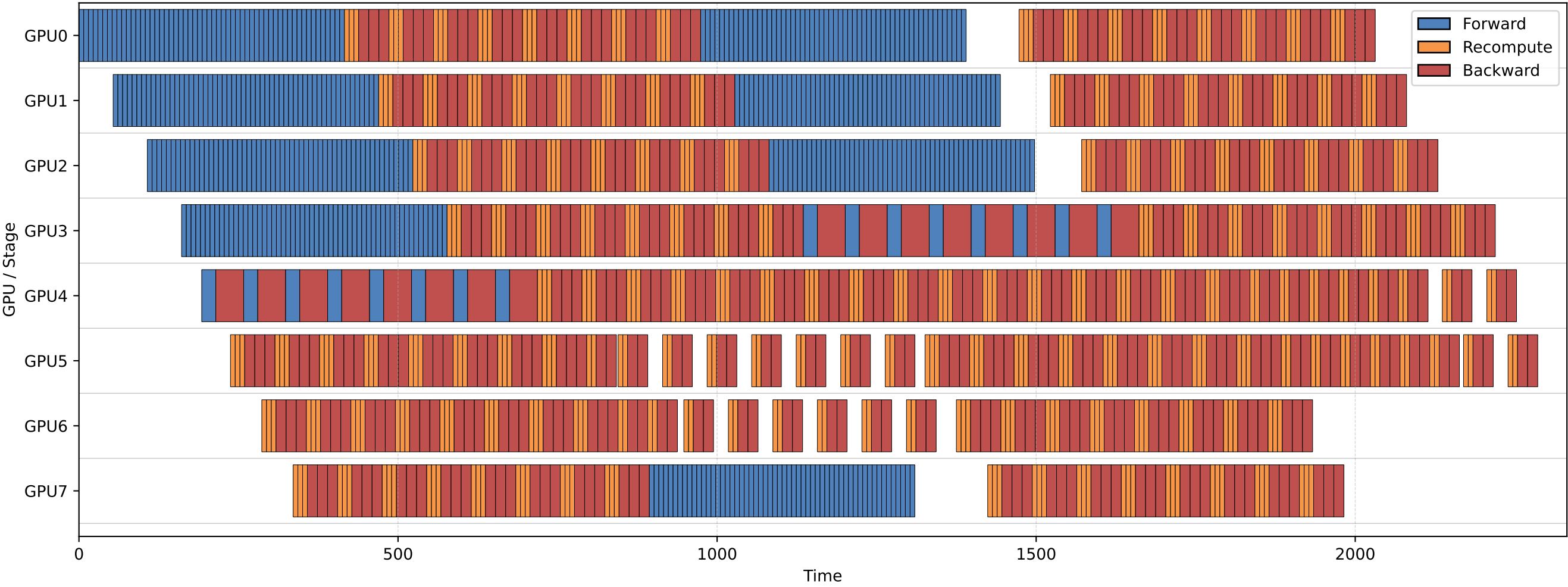
Qwen3-1.7B RoundPipe
