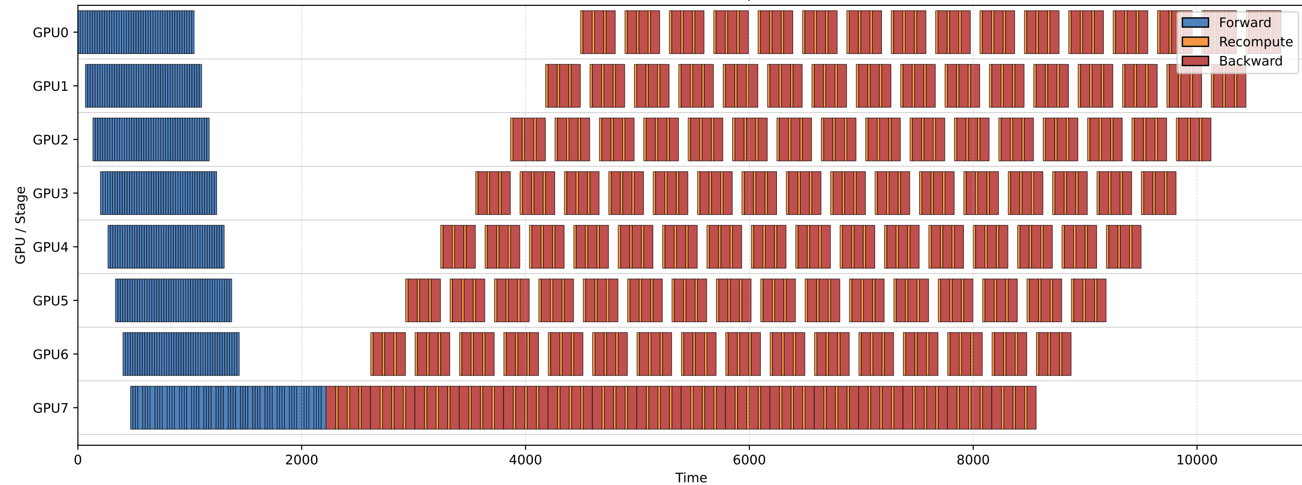
GPTOSS-20B GPipe
