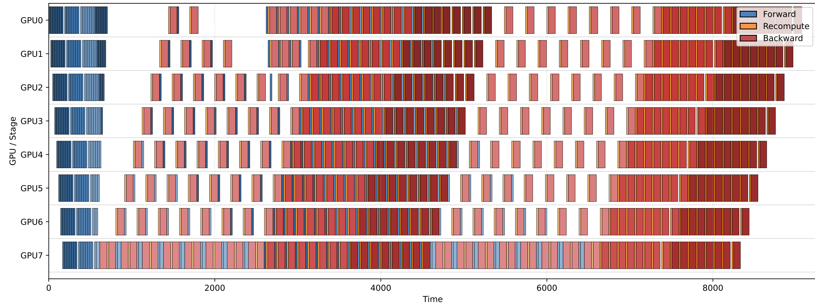
GPTOSS-20B Interleaved-1F1B
