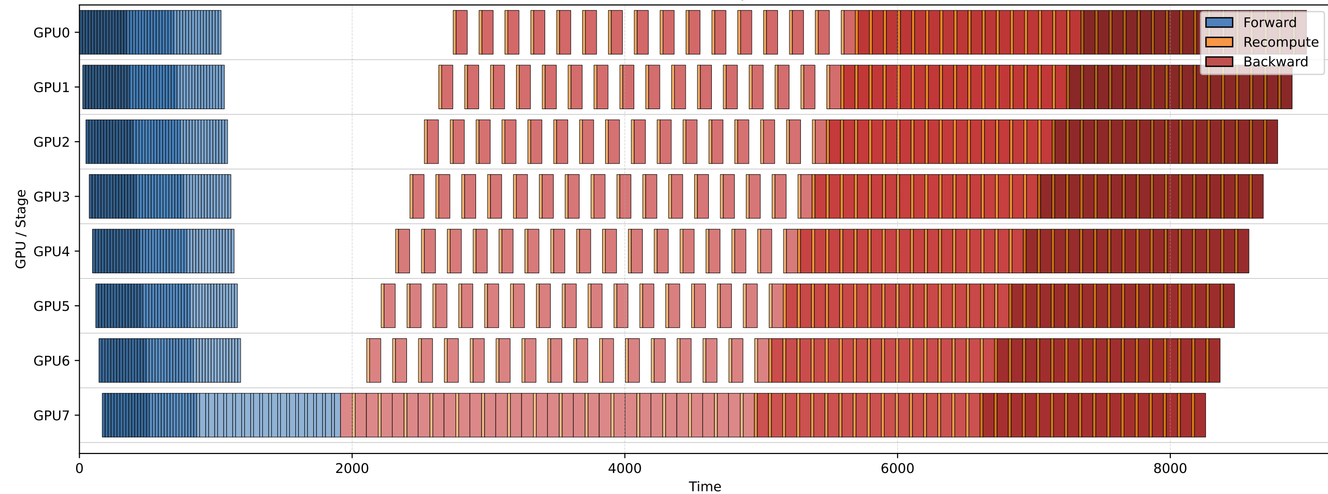
GPTOSS-20B Looped-BFS
