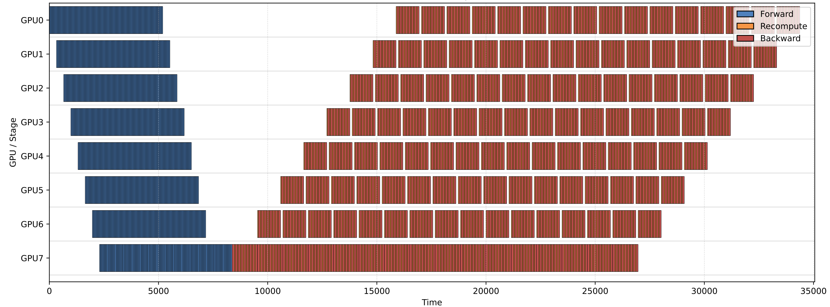
Qwen3-32B GPipe
