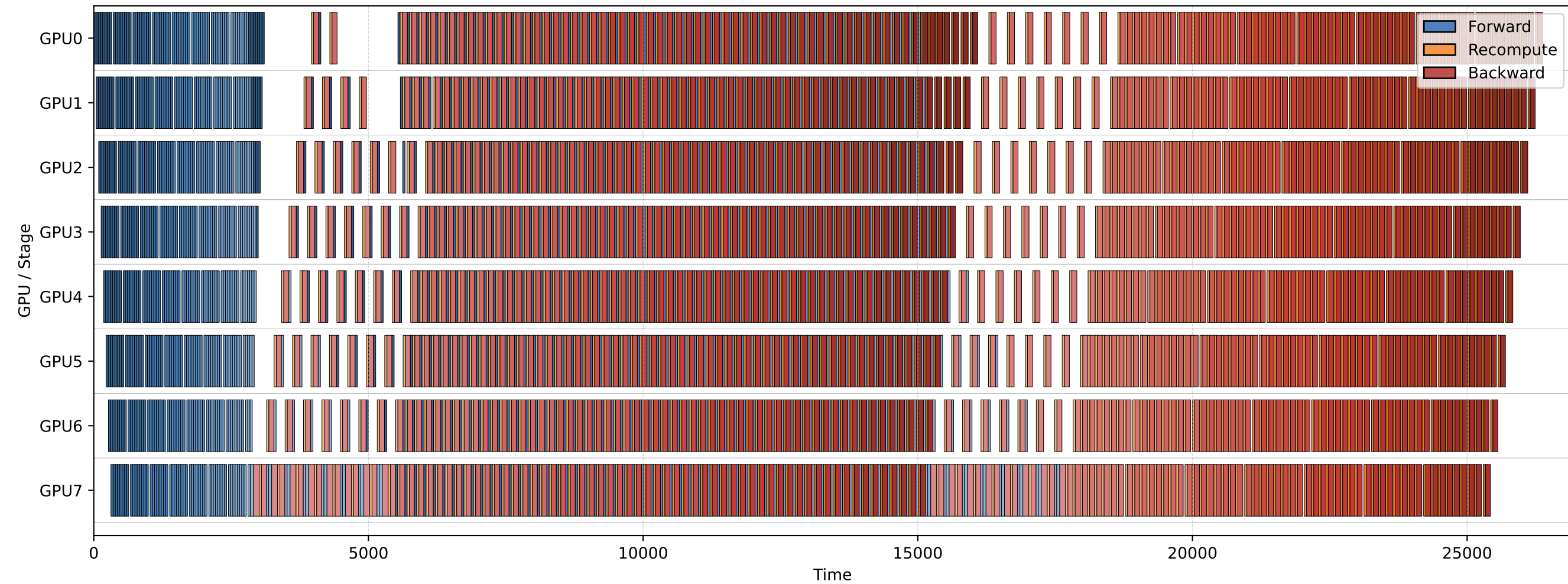
Qwen3-32B Interleaved-1F1B
