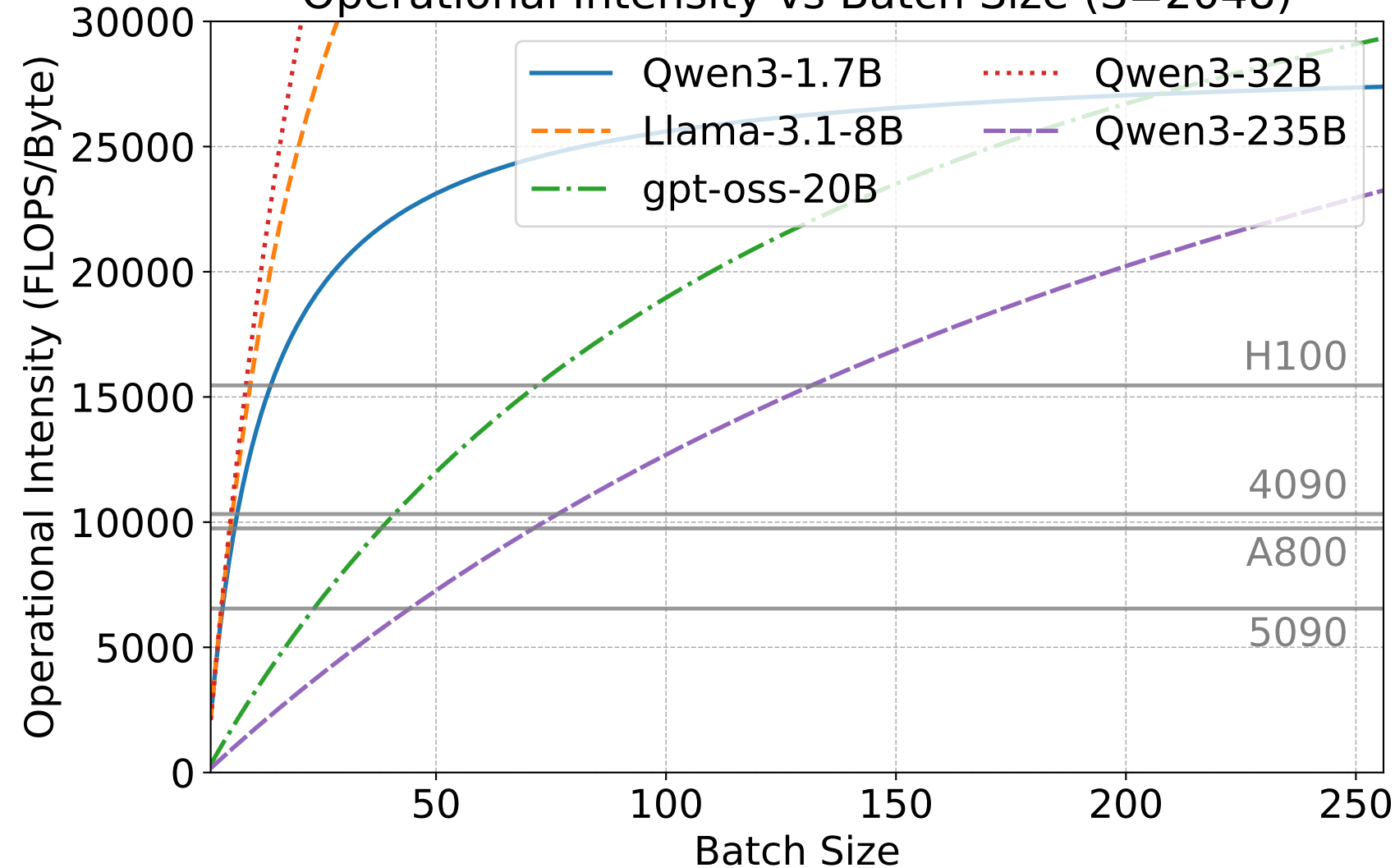
Operational Intensity vs Batch Size (S=2048)
