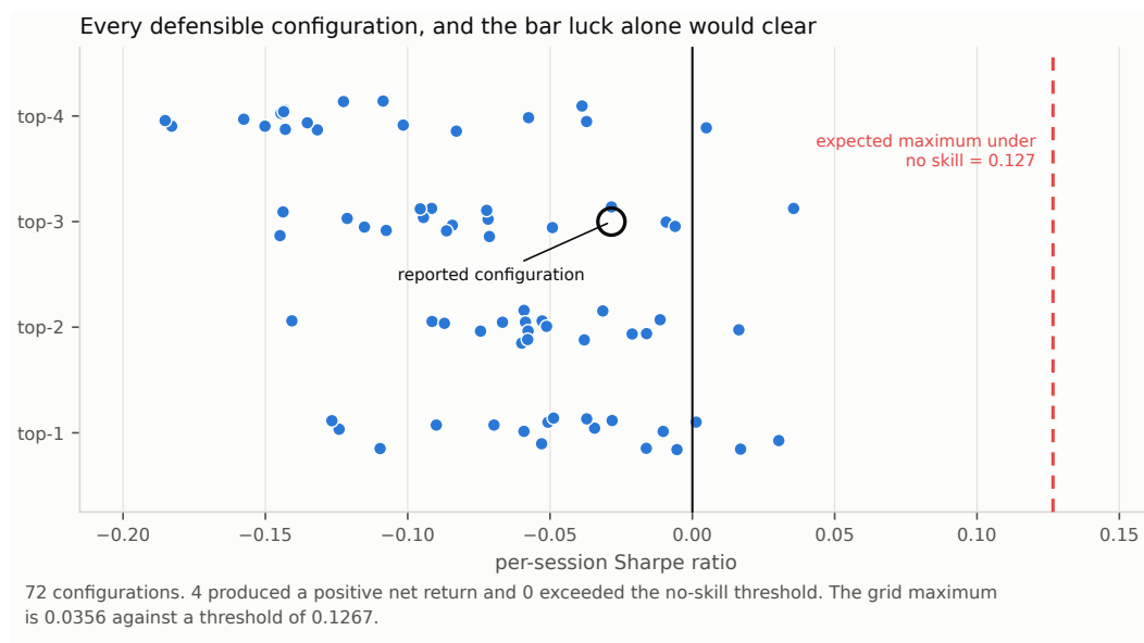
Figure 6: Every configuration in the grid against the Sharpe ratio that skill-free search alone would be expected to produce. The grid maximum does not reach the bar luck sets.
