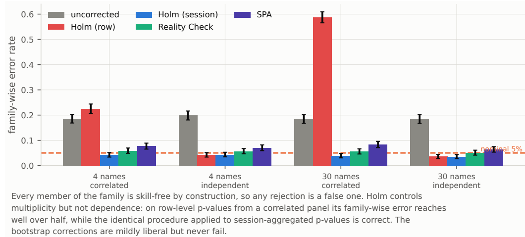
Figure 5: Family-wise error with every family member skill-free by construction. Holm applied to row-level p-values on a correlated panel fails; the same procedure on session-aggregated p-values is correct.
