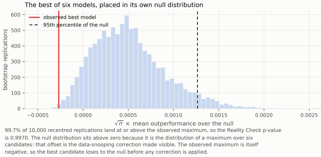
Figure 5: The best of six models placed inside its own bootstrap null distribution. The null is centred above zero because it is the distribution of a maximum over six candidates: that offset is the data-snooping correction made visible. The observed maximum is negative.
