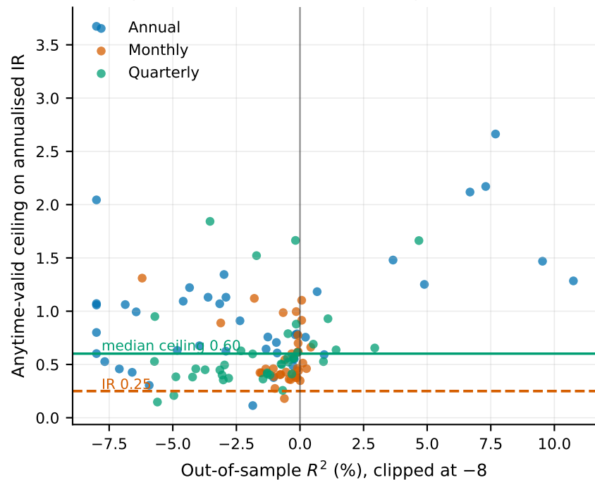
All 116 predictors, and how much they could still be worth
