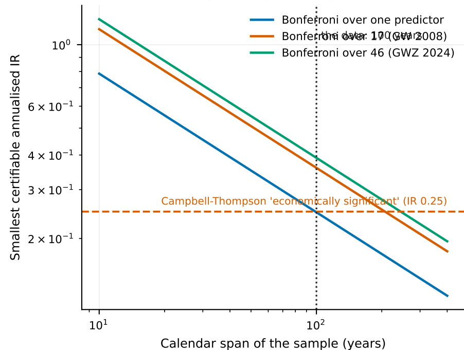
What a sample of a given length can settle
