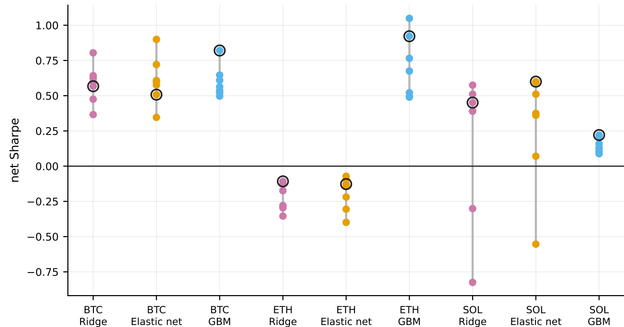
Sensitivity to the trading schedule's start offset ( h = 7d )
