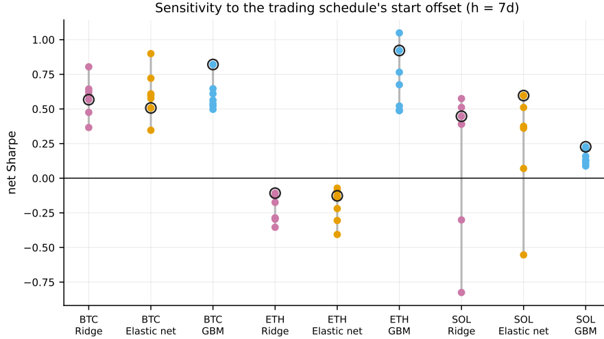
Figure 9: At h = 7 the single-phase backtest has seven possible starting offsets. Each bar spans the Sharpe ratios they produce for one setting. The spread reaches 1.40 points, which is larger than any difference between models, and it is why the primary specification holds all seven vintages at once rather than choosing among them.
