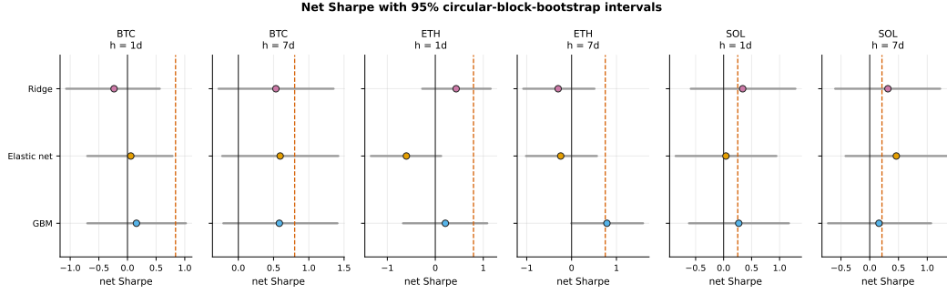
Figure 8: Net Sharpe with 95% circular-block-bootstrap intervals (10,000 resamples), under the primary specification: an equal-weighted portfolio over all h daily vintages, entered one bar after the signal is observable. The dashed line marks buy-and-hold on the same schedule and cost model. No interval excludes zero.
