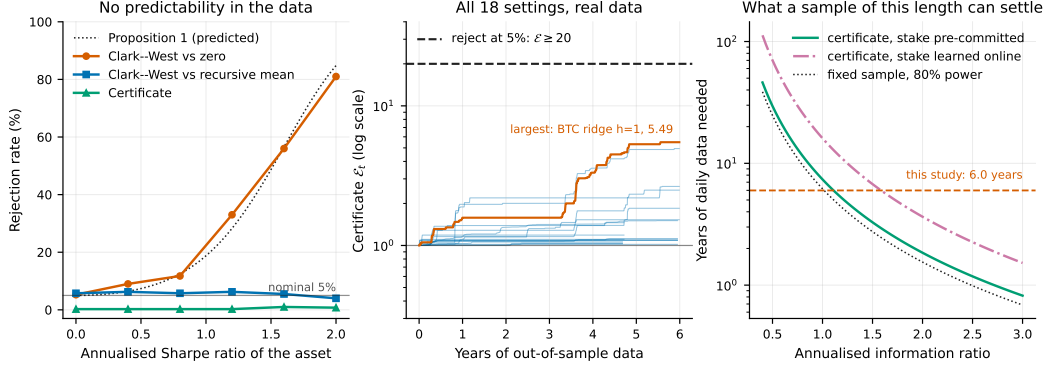
Figure 1: The argument in three panels. Left: rejection rate on data containing no conditional predictability, as the asset’s drift grows. Clark–West against a zero benchmark climbs from nominal to 81%, tracking the closed form of Proposition 1 (dotted); against the recursive mean it is correctly sized in this design; the certificate is bounded by its nominal level uniformly in the drift, which is Theorem 2. Middle: every certificate this study produces, against the threshold it would have to cross. The largest reaches 1.82 where 20 is required. Right: the detection-horizon law of Theorem 8. Six years of daily data—about what any liquid cryptocurrency offers—sits below the curve for every information ratio under 1.6, so those effects are out of reach at this sample size whatever the test.
