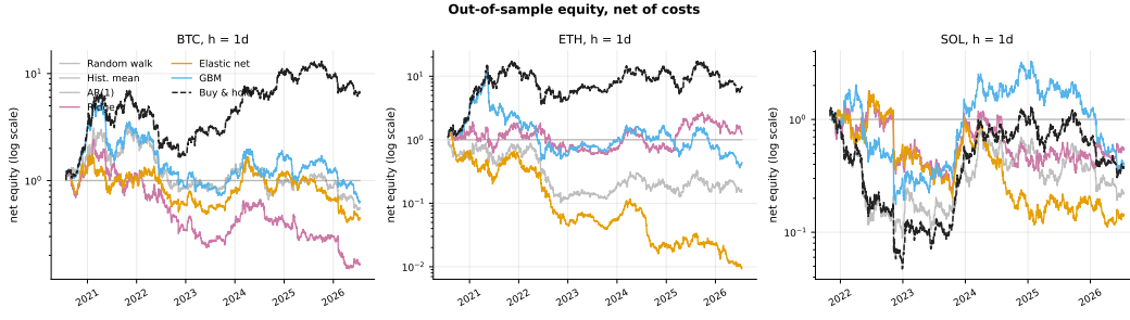
Figure 10: Out-of-sample equity net of costs at h = 1 , against the always-long reference on the same schedule and cost model. Starting capital is unity and the vertical scale is logarithmic.
