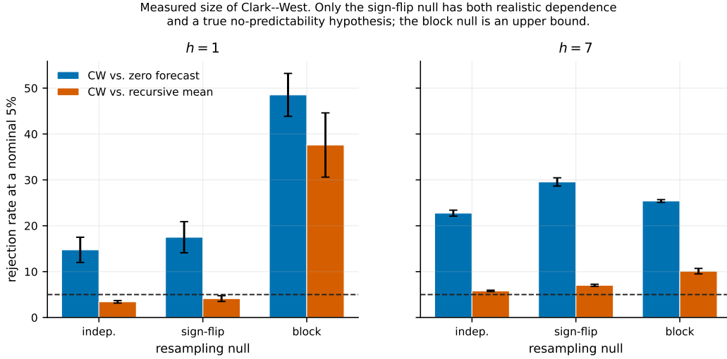
Figure 3: Measured rejection rate at a nominal 5% under the three resampling nulls. Bar height averages the estimators measured in each cell and the whisker spans them. Only the sign-flip null has both realistic dependence and a true no-predictability hypothesis; the block null is an upper bound on size. The gap between them is consistent with dependence the block bootstrap retains and sign randomisation removes; Table 5 shows that conditional mean dependence is one candidate among several, and a GARCH null that shares neither generator’s artifacts gives the same answer.
