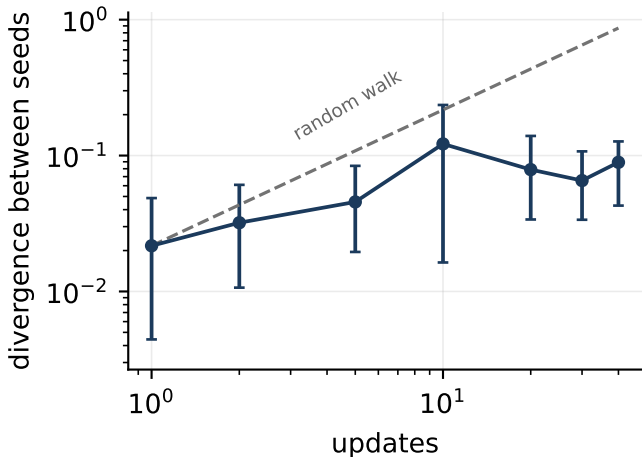
Qwen2.5-0.5B, 6 seeds
