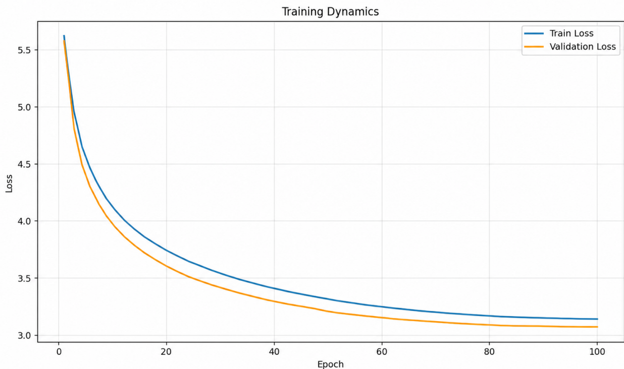
Fig. 5.11. Training dynamics of the CSU-MS2 model.
