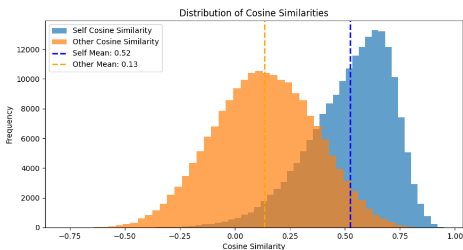
Fig. 5.12. Distribution of self-similarity and random-similarity values for the JESTR model.
