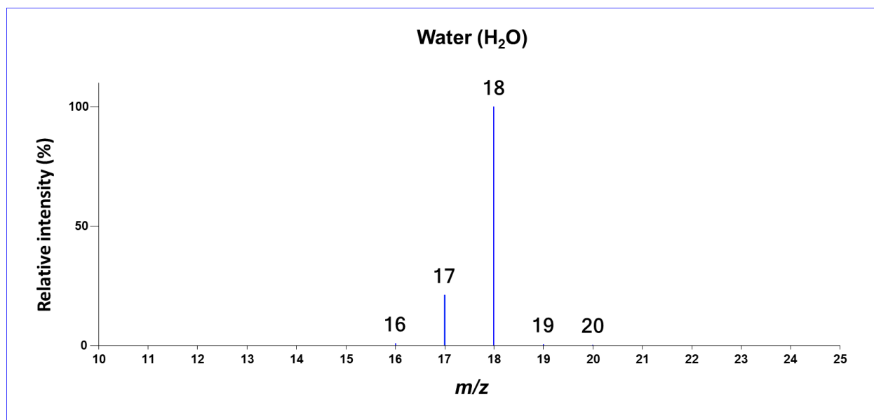
Fig. 2.3. Example of mass spectrum diagram. Adapted from JEOL USA Mass Spectrometry Basics [17].
