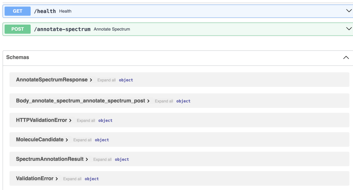
Fig. 5.21. FastAPI interface with available endpoints and response schemas.
