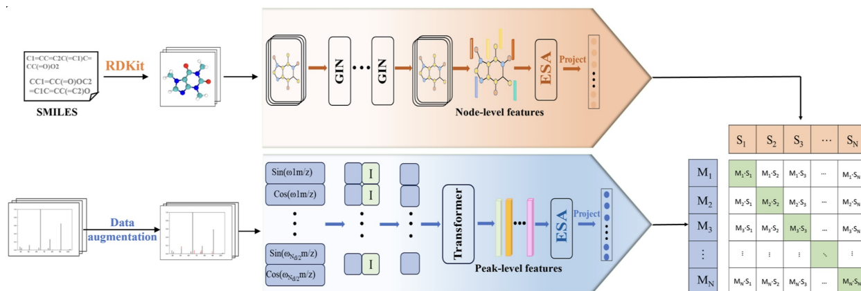
Fig. 5.10. Architecture of the CSU-MS2 model, integrating transformer-based spectral encoding, graph neural network-based molecular encoding, and ESA-based cross-modal aggregation.
