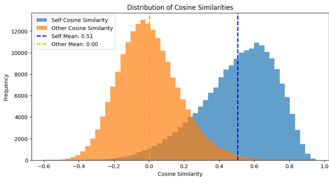
Fig. 5.14. Distribution of self-similarity and random-similarity values for the CSU-MS2 model.
