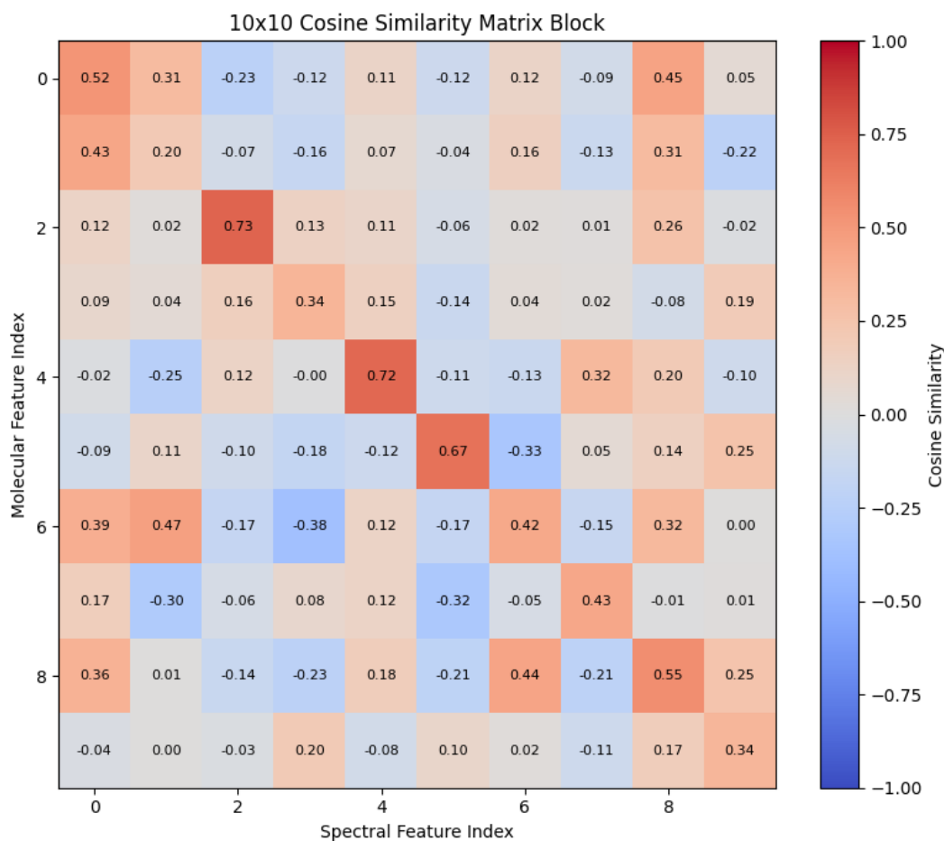
Fig. 5.15. Local 10 \times 10 cosine-similarity matrix block for the CSU-MS2 model.
