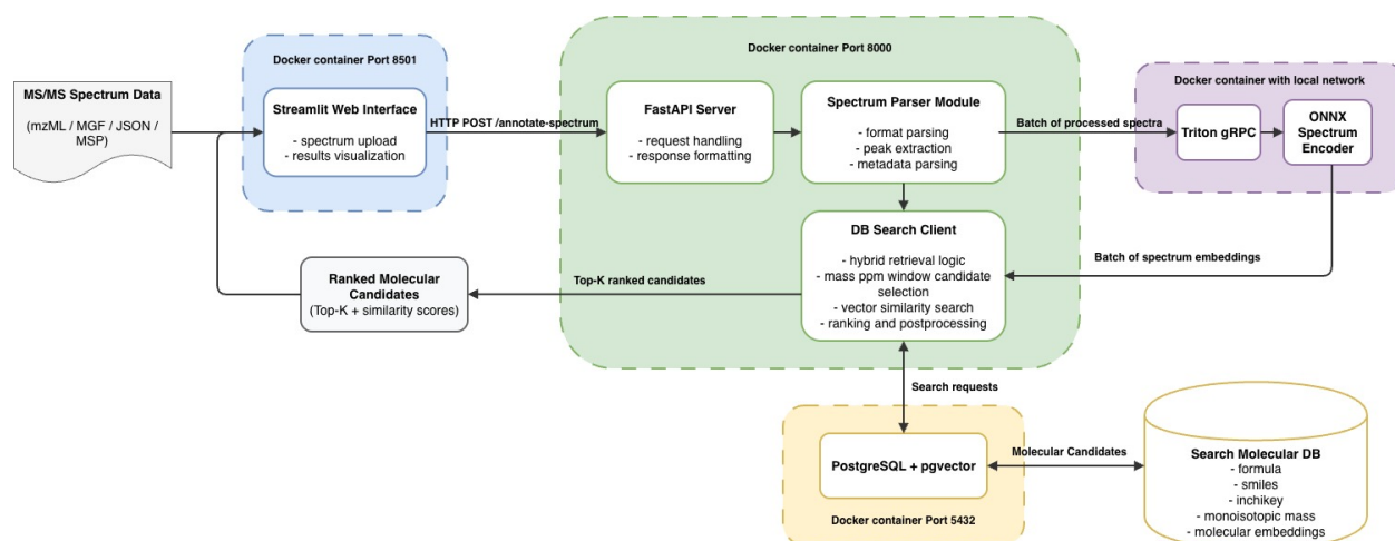
Fig. 4.1. System architecture of the proposed spectrum–molecule retrieval system.
