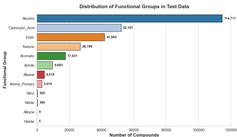
Fig. 5.3. Distribution of functional groups in the test dataset.
