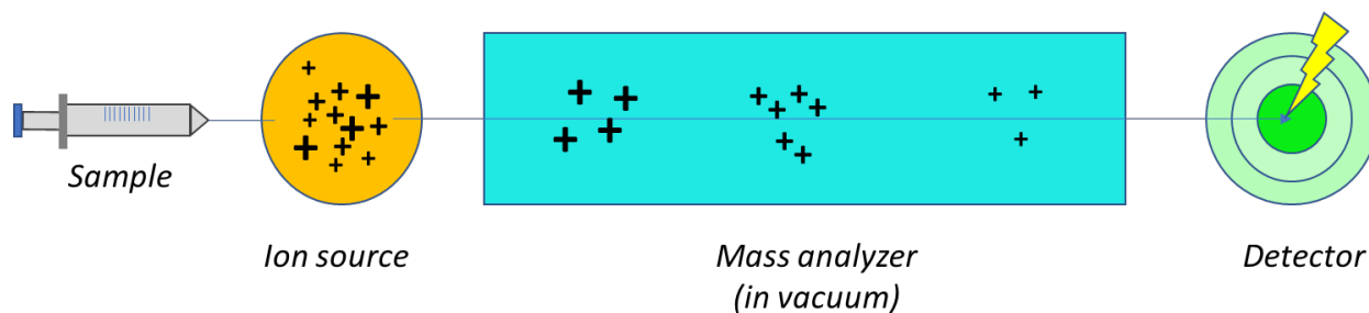
Fig. 2.1. General principle of mass spectrometry, illustrating analyte ionization, ion separation according to mass-to-charge ratio ( m/z ), and spectrum generation through ion detection. Adapted from JEOL USA Mass Spectrometry Basics [17].
