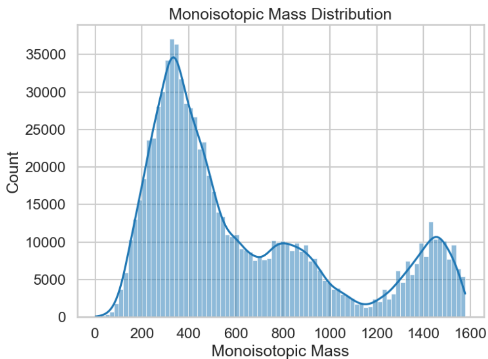
Fig. 5.5. Distribution of monoisotopic mass in the molecular database.
