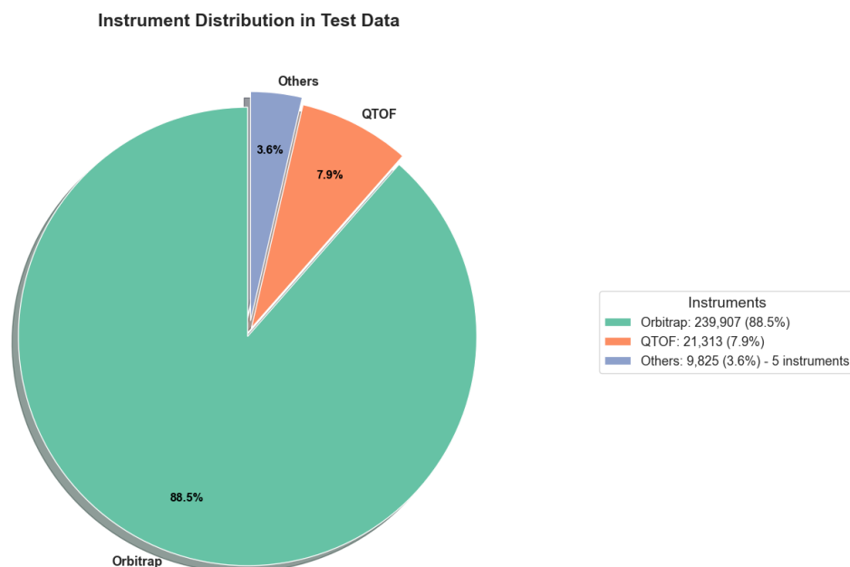
Fig. 5.4. Distribution of instruments in the test dataset.
