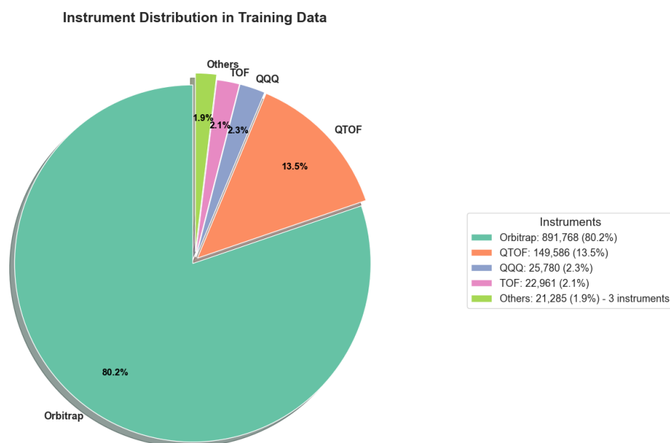
Fig. 5.2. Distribution of instruments in the training dataset.
