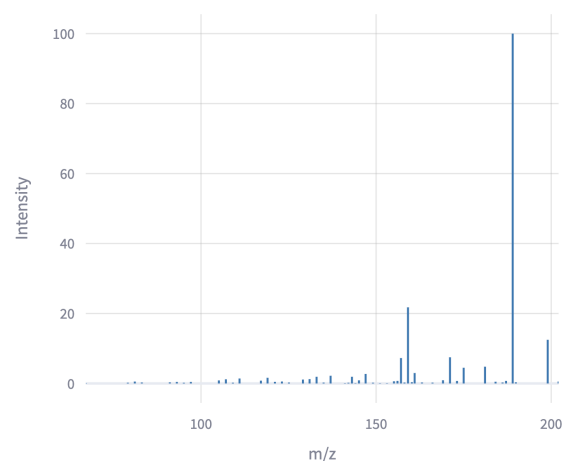
Fig. 5.18. Visualization of uploaded spectra in preview mode.
