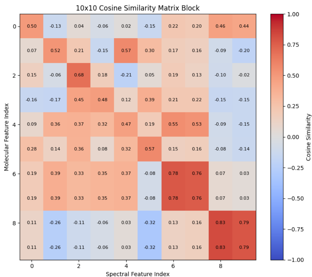
Fig. 5.13. Local 10 \times 10 cosine-similarity matrix block for the JESTR model.
