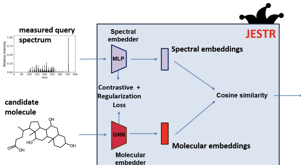
Fig. 5.8. Architecture of the JESTR model. The model follows a dual-encoder design with independent spectrum and molecule encoders and similarity-based matching in a shared latent space.
