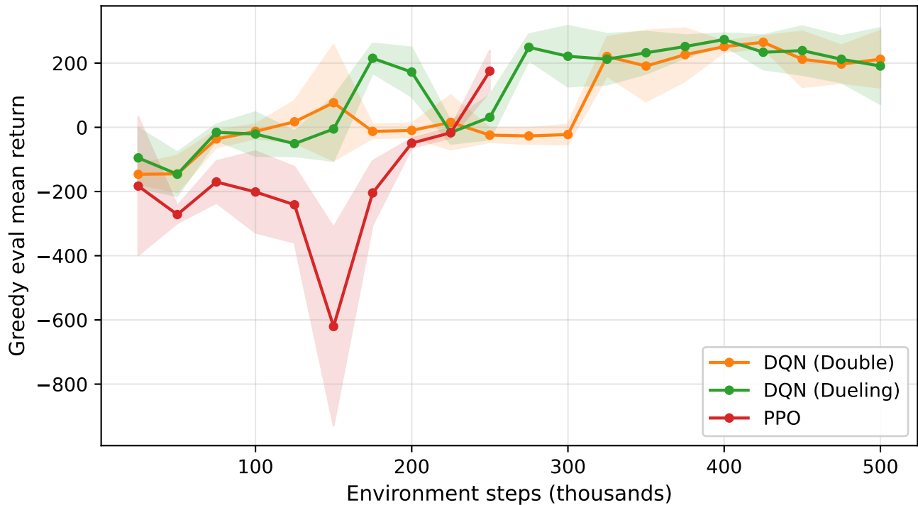
LunarLander: greedy evaluation curve
