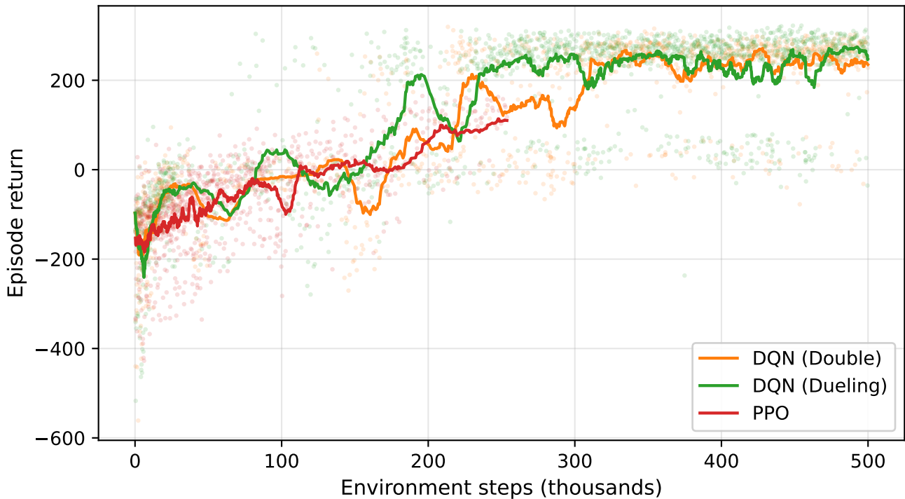
LunarLander: training-time episode return (30-ep MA)
