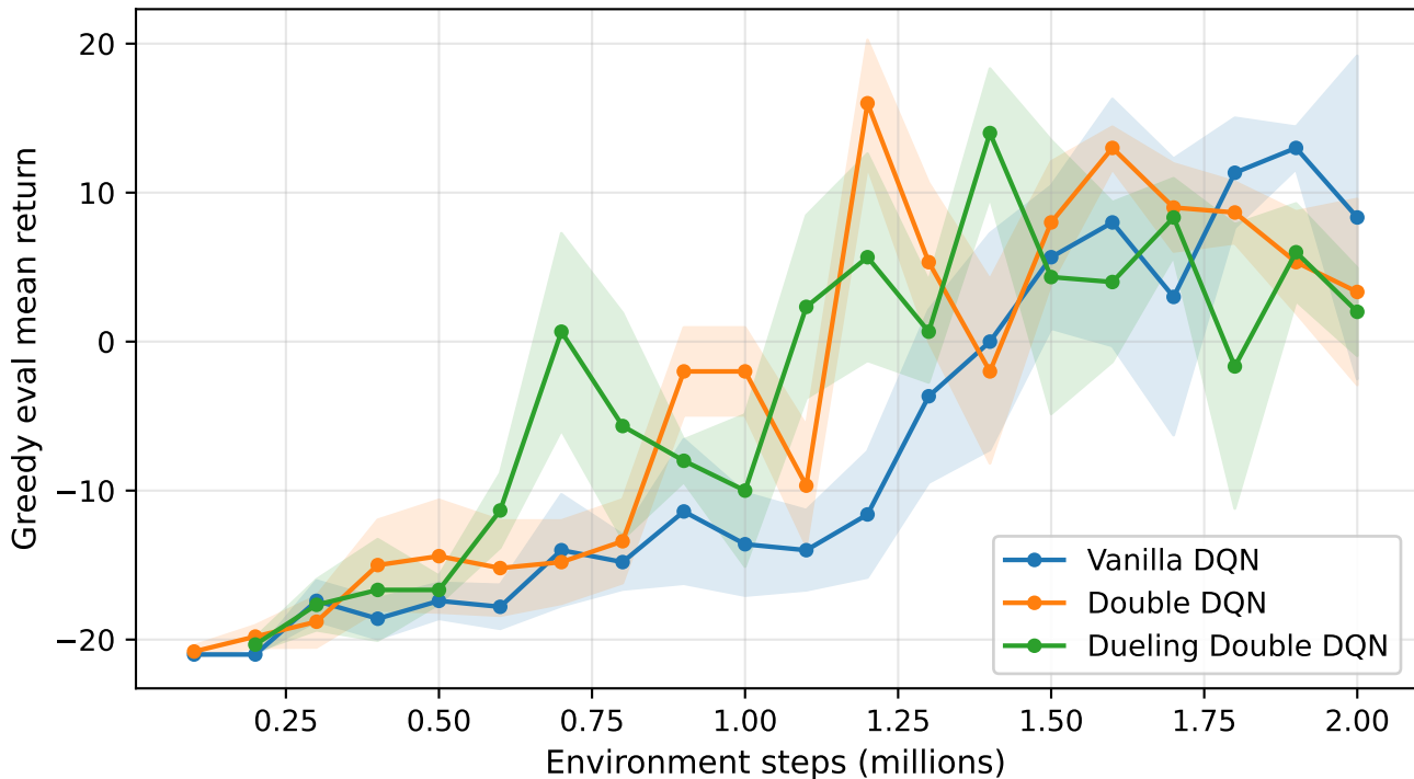
Pong: greedy evaluation (5 eps/checkpoint)
