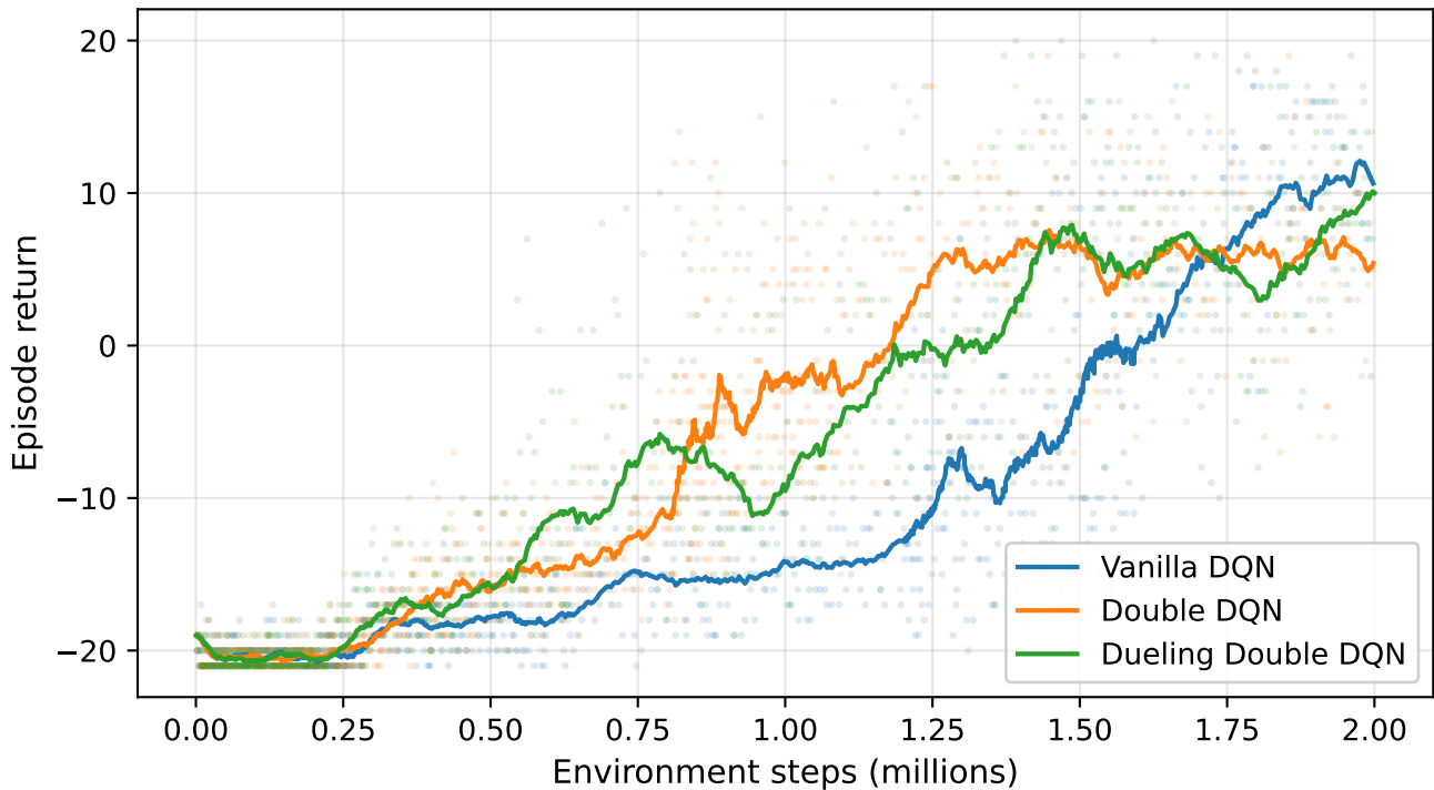
Pong: training-time episode return (30-ep MA)
