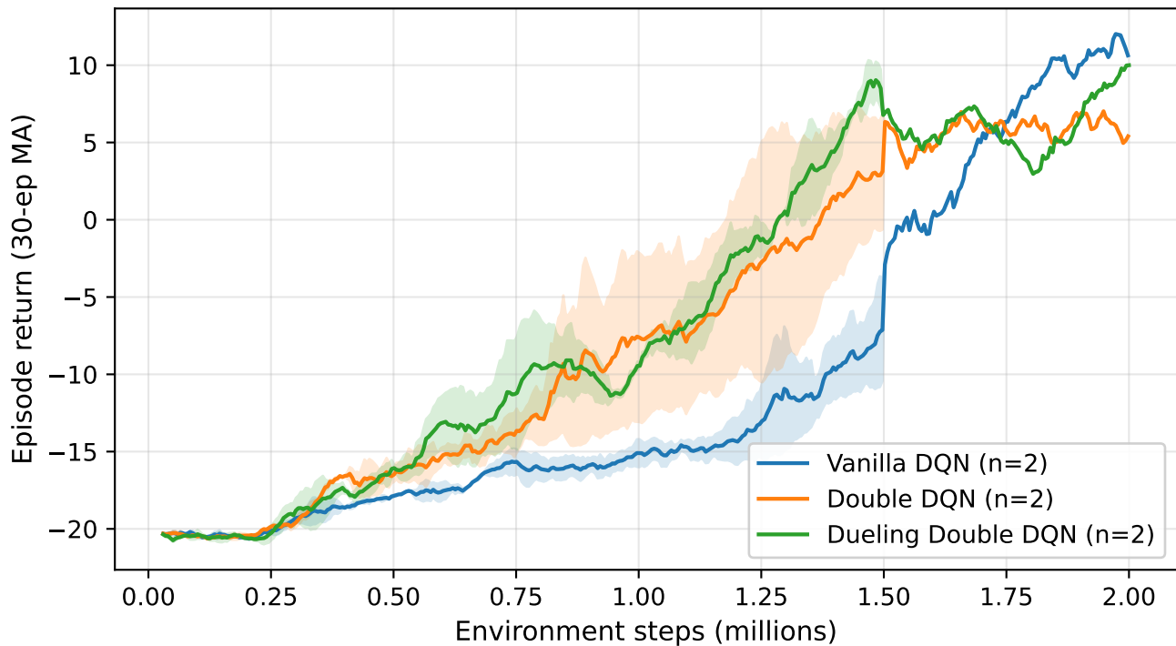
Pong: training-time return, multi-seed (mean \pm std)
