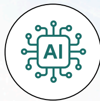
Artificial Intelligence
