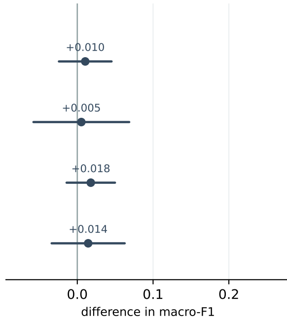
hyperedge over graph (hypergraph – pairwise)
