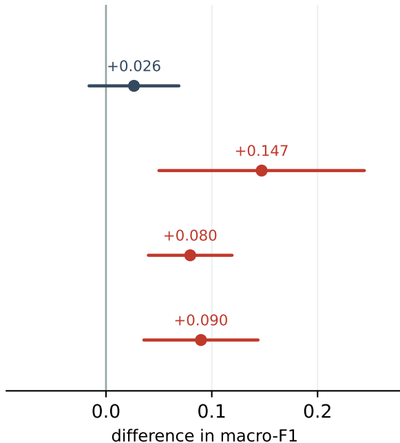
graph over composition (pairwise – composition)
