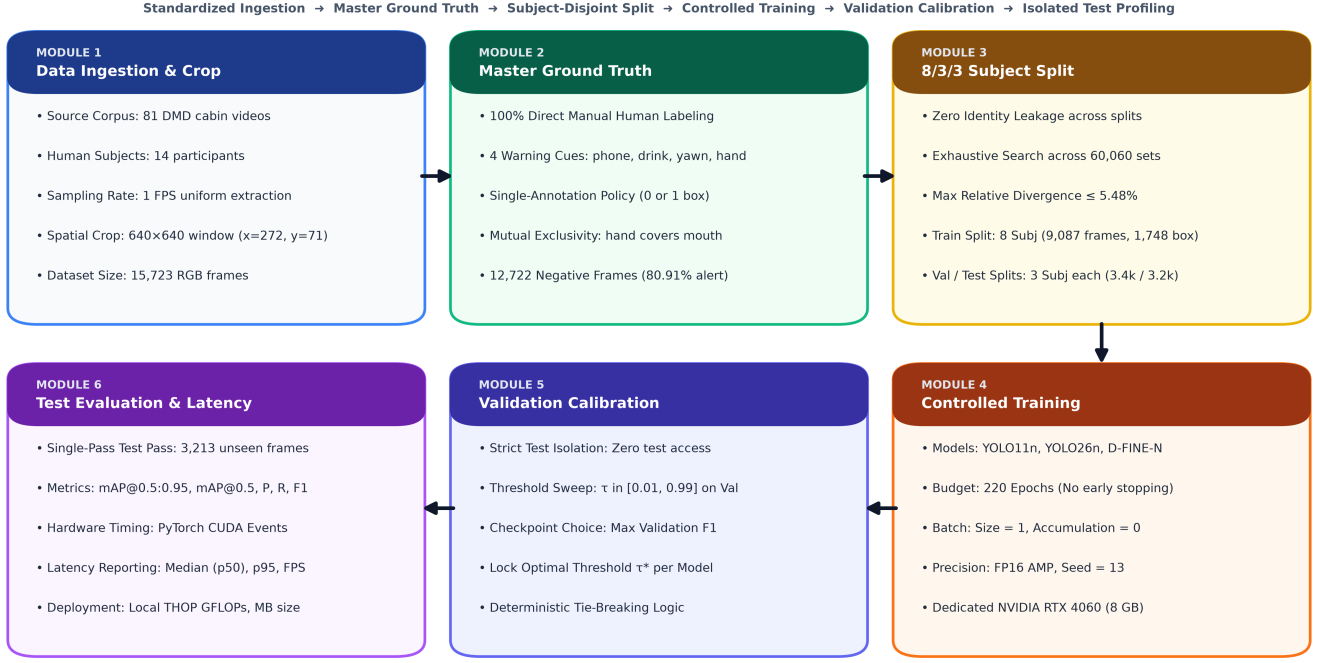
Fig. 4. DMS-Eval end-to-end benchmark framework and evaluation lifecycle: spanning standardized 640 × 640 frame extraction from 81 DMD videos, authoritative Label Studio ground truth annotation across 4 target visual warning cues (80.91% negative frames), deterministic 8/3/3 subject-disjoint split optimization ( \leq 5.48\% relative divergence), controlled training on RTX 4060 hardware (batch size 1, 220 epochs, seed 13), validation-only F_1 score threshold calibration ( \tau^* ), and isolated single-pass test evaluation.
