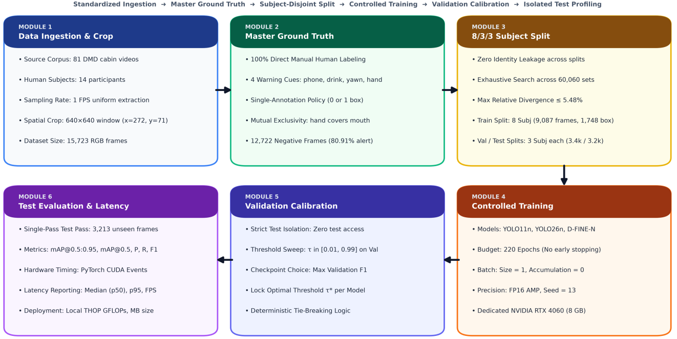
Fig. 4. DMS-Eval end-to-end benchmark framework and evaluation lifecycle: spanning standardized 640 \times 640 frame extraction from 81 DMD videos, authoritative Label Studio ground truth annotation across 4 target visual warning cues (80.91% negative frames), deterministic 8/3/3 subject-disjoint split optimization ( \leq 5.48\% relative divergence), controlled training on RTX 4060 hardware (batch size 1, 220 epochs, seed 13), validation-only F_1 score threshold calibration ( \tau^* ), and isolated single-pass test evaluation.
