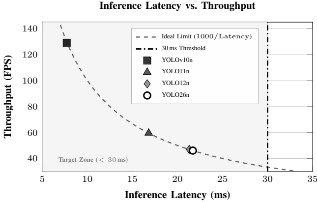
Fig. 3. Inference latency versus throughput across the evaluated YOLO models. Each model uses a distinct marker shape for greyscale clarity. The dashed vertical line marks the 30 ms real-time deadline.
