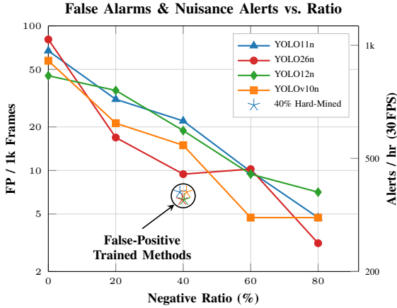
Fig. 5. Measured false-positive rates (left axis) and projected hourly alerts at 30 FPS (right axis; via (6)) versus negative ratio. Both axes share synchronized log scales due to the linear relation ( \mathcal{A}_h = 87.4 \times \text{FP/1k} ). The circled cluster highlights 40% hard-negative mining results; star markers are jittered (39.0–41.0) for visual separation only, all four represent the identical 40% ratio.
