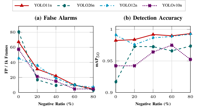
Fig. 4. Impact of negative-to-positive curation ratios (RQ1): (a) false alarms per 1,000 frames (FP/1k) across curation ratios; (b) core detection accuracy (mAP 50 ). Distinct marker shapes and line styles provide visual encoding for greyscale readability.
