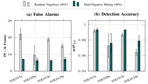
Fig. 6. Hard-negative mining versus random negative sampling ( r_{\text{ref}} = 40\% , RQ2): (a) false alarms per 1,000 frames (FP/1k); (b) core detection accuracy ( \text{mAP}_{50} ). Bars report dual-seed sample means with \pm 1 standard deviation error bars.
