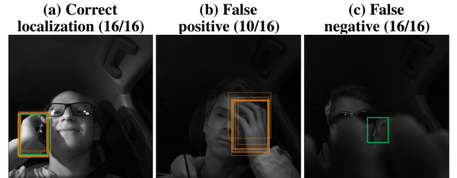
Fig. 4. Agreement-selected NIR outcomes at frozen thresholds. Green denotes ground truth and orange denotes predictions. The correct localization and false negative are unanimous; the most recurrent negative-frame false positive occurs in 10/16 runs.
