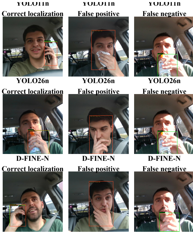
Fig. 3. Representative seed-13 outcomes for YOLO11n, YOLO26n, and D-FINE-N. Green boxes denote ground truth and orange boxes denote predictions at the validation-selected threshold; columns show a correct localization, a false detection on a nominal negative, and a false negative.
