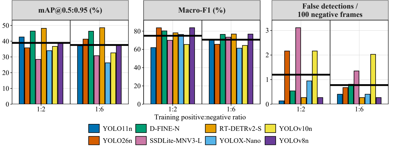
Fig. 5. Sixteen NIR protected-test results at seed 13 and deterministic 1-FPS midpoint sampling. Distinct colors identify the eight models at 1:2 and 1:6 training exposures; the dark-grey rule separates the ratio sections, and each thick black segment marks the eight-model mean for its ratio.
