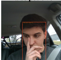
D-FINE-N
