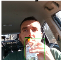
D-FINE-N
