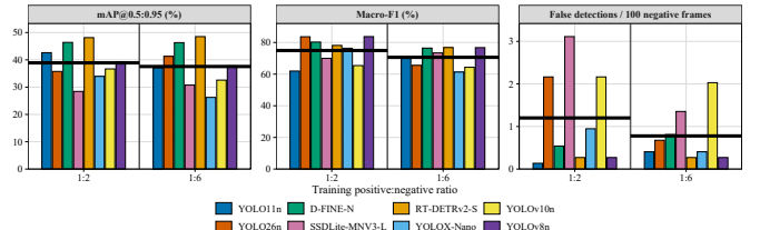
Fig. 5. Sixteen NIR protected-test results at seed 13 and deterministic 1-FPS midpoint sampling. Distinct colors identify the eight models at 1:2 and 1:6 training exposures; the dark-grey rule separates the ratio sections, and each thick black segment marks the eight-model mean for its ratio.
