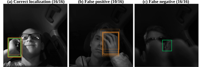
Fig. 4. Agreement-selected NIR outcomes at frozen thresholds. Green denotes ground truth and orange denotes predictions. The correct localization and false negative are unanimous; the most recurrent negative-frame false positive occurs in 10/16 runs.
