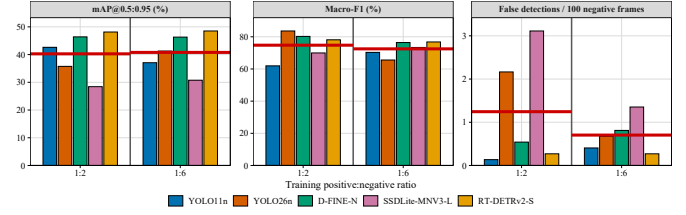
Fig. 4. Ten NIR protected-test results at seed 13 and deterministic 1-FPS midpoint sampling. Grouped columns compare each completed model at 1:2 and 1:6 training exposures; the dark-grey rule separates the ratio sections, and each thick red segment marks the five-model mean for its ratio.
